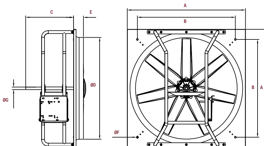
EXTRACTOR HGTA
