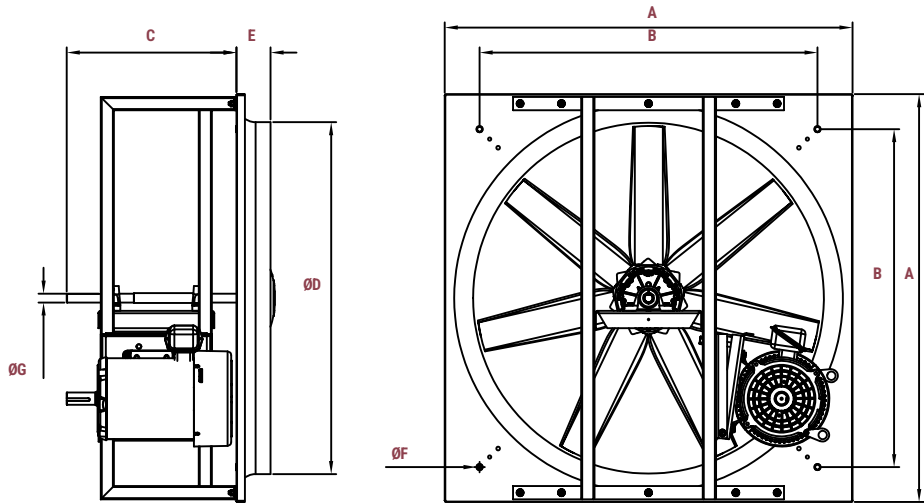
EXTRACTOR HGTA
